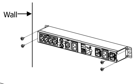
Chart 2: Wall mounting
